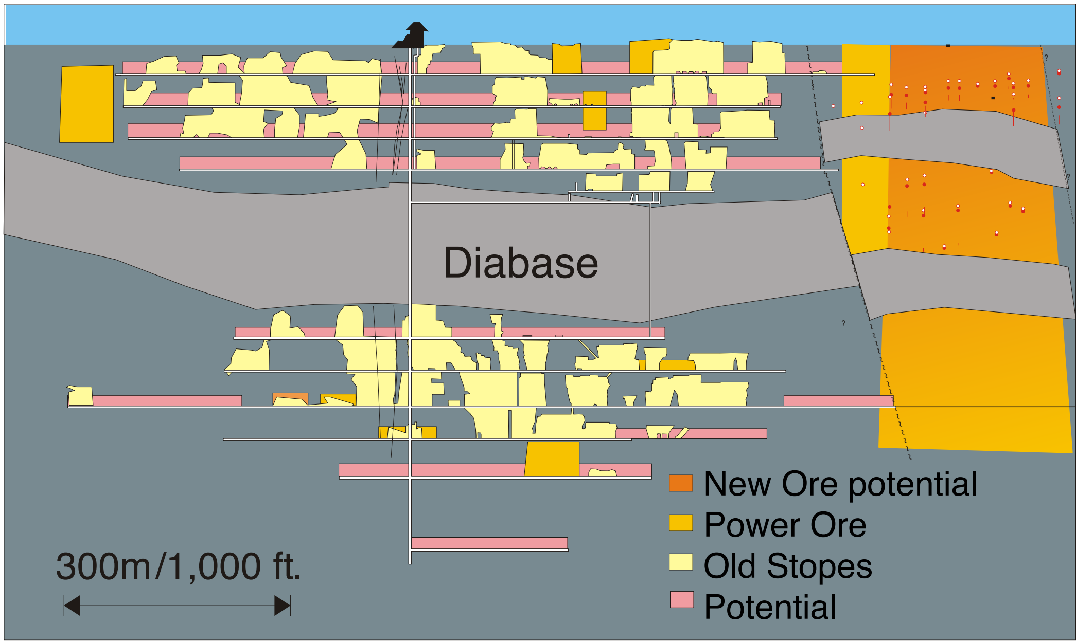
Northern Empire Mine longitudinal view
